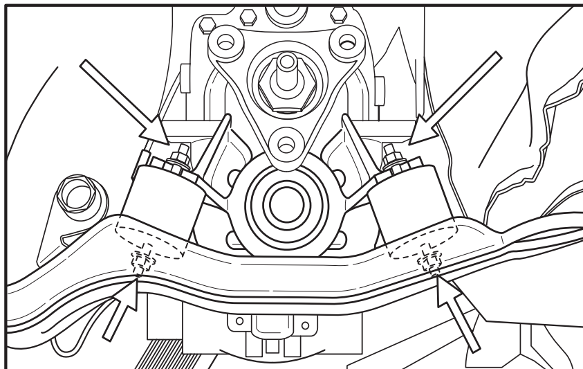
Cotsis CAD Illustration shows hidden bolts
